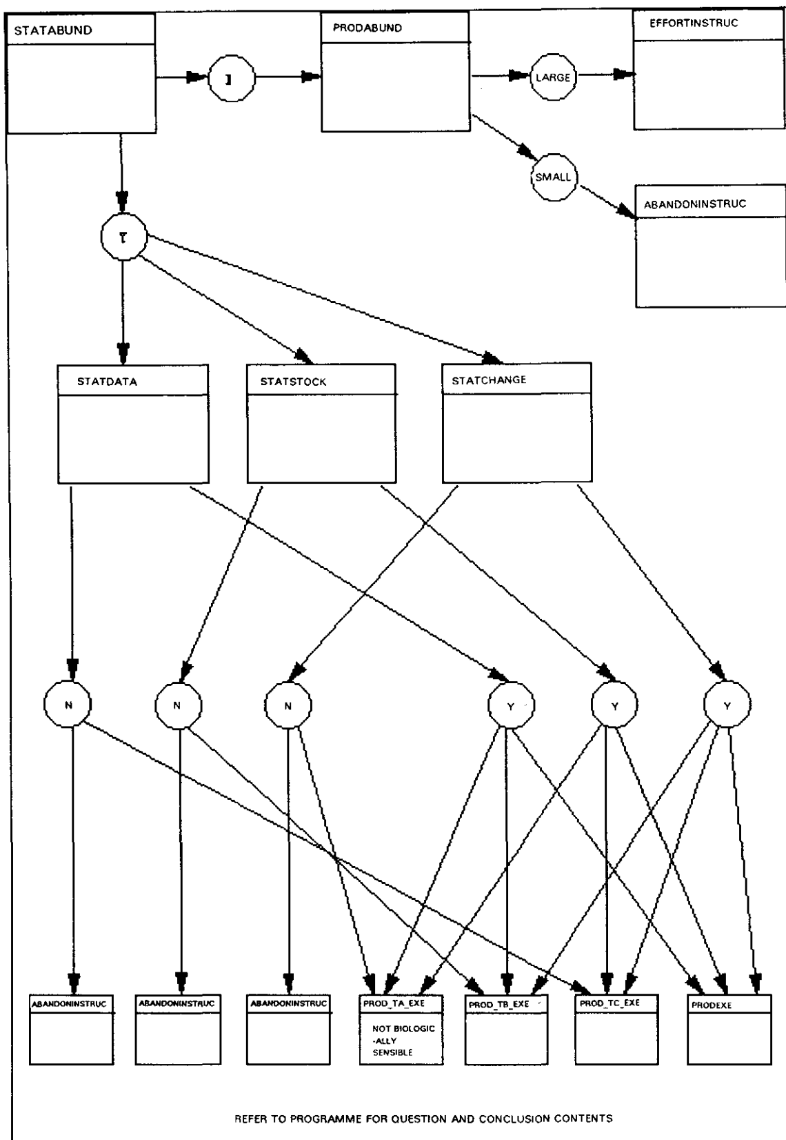
Figure 2 The ZPM. KB Production Modelling Expert System Decision Pathway
